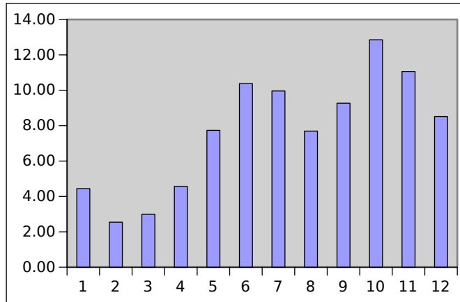
Precipitation (in)
